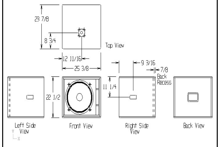
LF-118F All dimensions are in inches.
